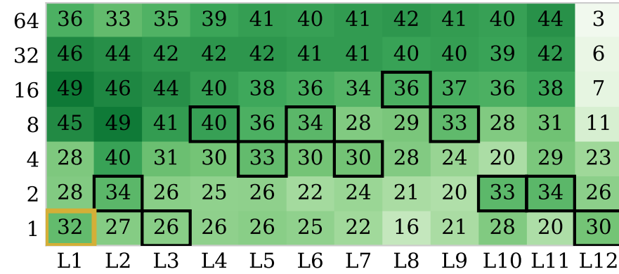
LaBraM
