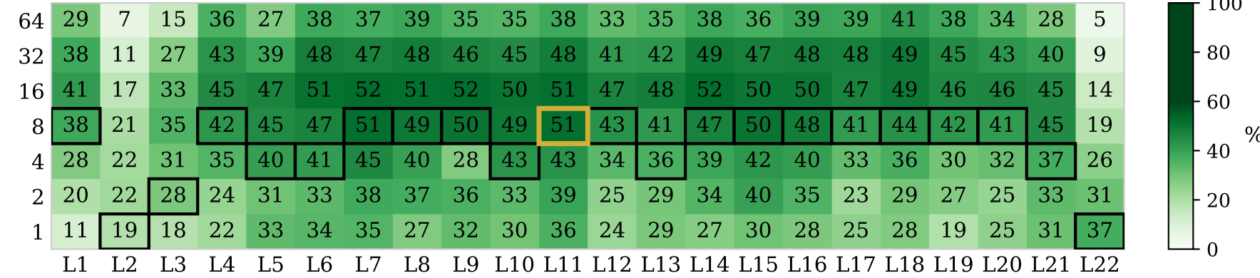
REVE
